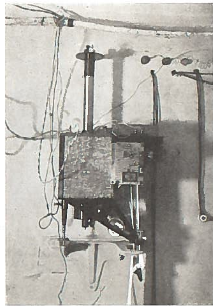
Fig. 17. Electrometer for recording of the potential gradient.
