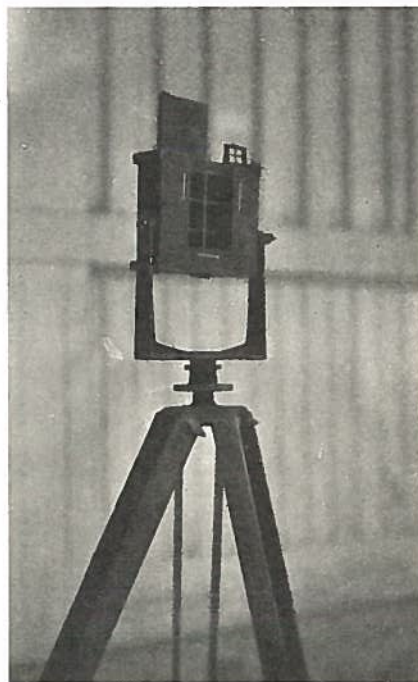
Fig. 14. Auroral Camera of the Störmer—Krogness type.
